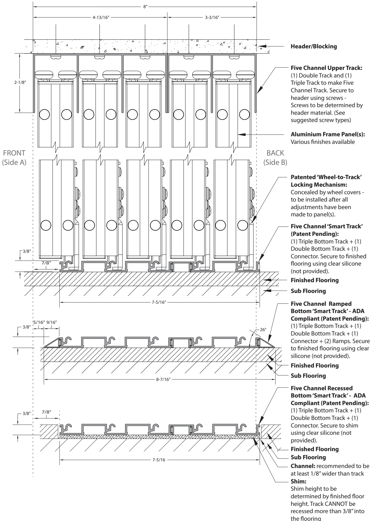
Sill Detail Opt. 2 at half scale Five Channel "Ramped" Bottom Track
