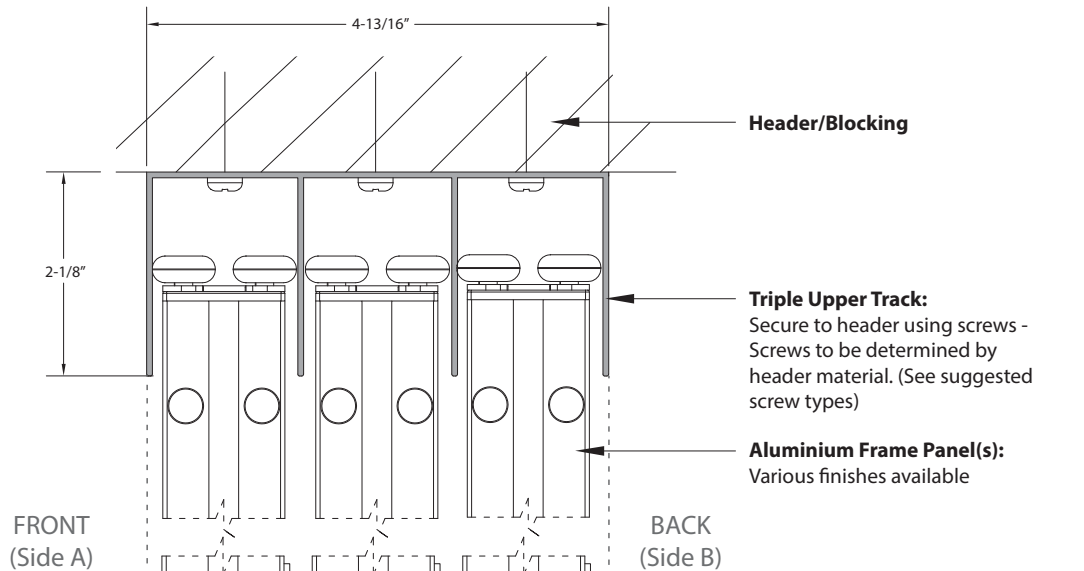
Header Detail at half scale Triple Upper Track
